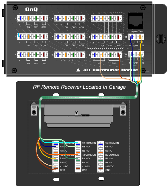
OnQ Part No. 364645-01 ALC Distribution Module Co-Located at Service Center with Controller
