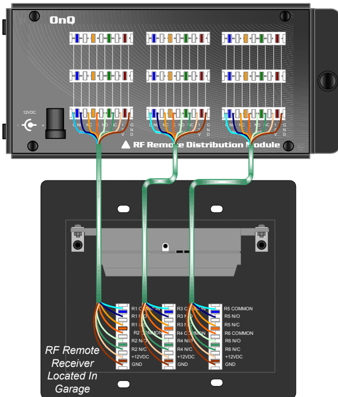
OnQ Part No. 364696-01 RF Remote Distribution Module Co-Located at Service Center with Controller
