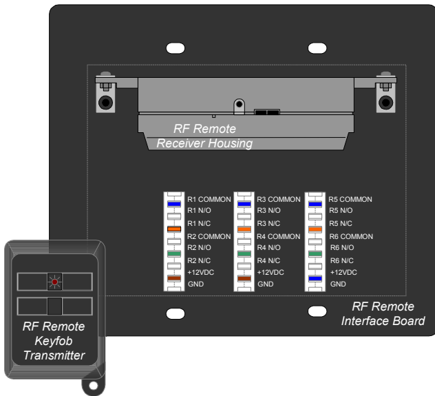
Figure 1. RF Remote Control Combo
