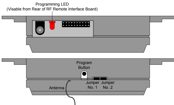
Figure 2. RF Remote Receiver Programming Features
